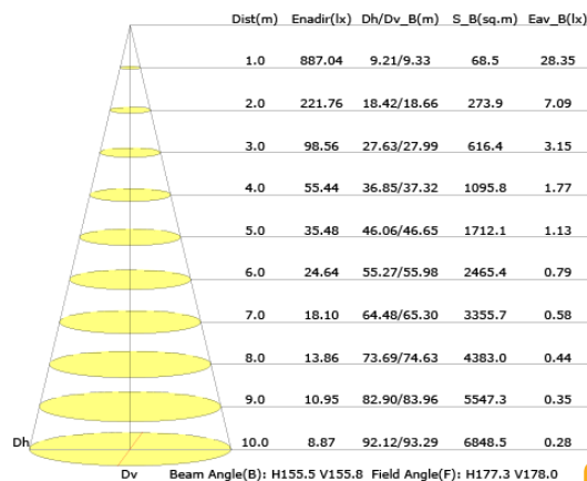
The Average Illuminance Effective Figure
