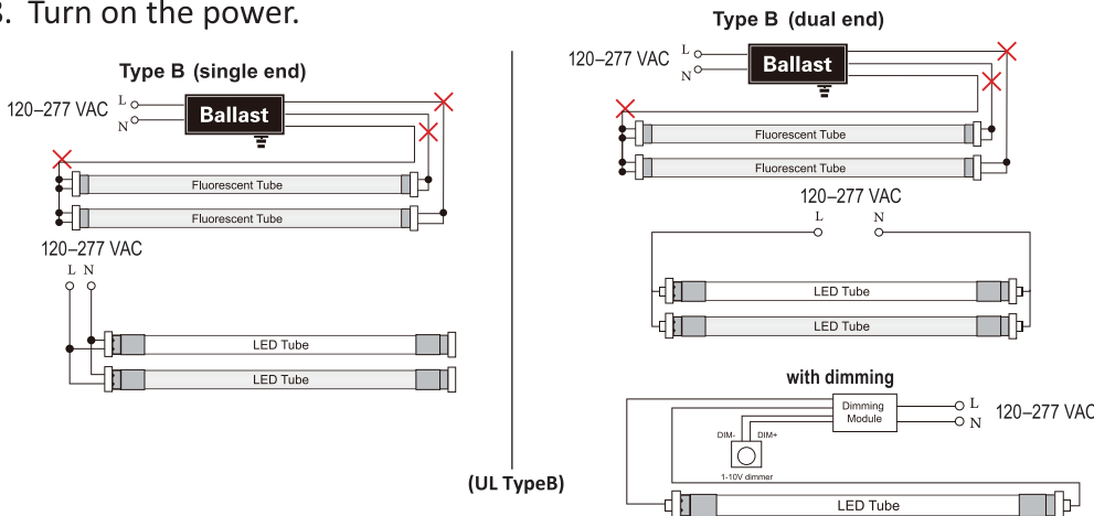
Shunted vs. non-shunted sockets Path of electrical current in red
