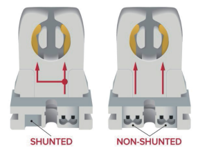
Shunted socket is required in double end mode
